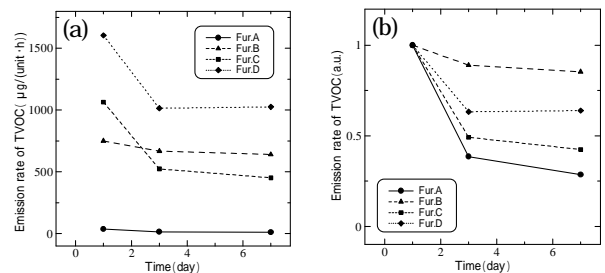
Fig.2 Characteristics of emission rate of TVOC. (b) represents (a) normalized by emission rate at 1 day.
