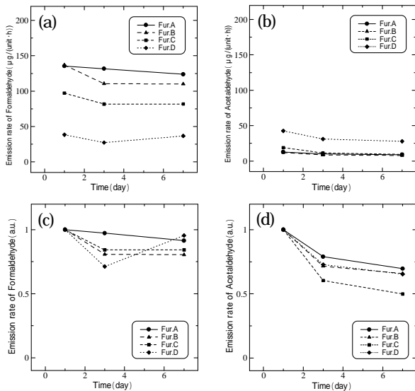
Fig. 1 Characteristics of emission rate of aldehydes. (c) and (d) represent (a) and (b) normalized by emission rate at 1 day, respectively.
