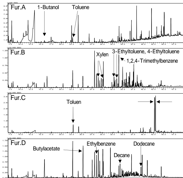
Fig. 3 TIC of each furniture at 1 day.
